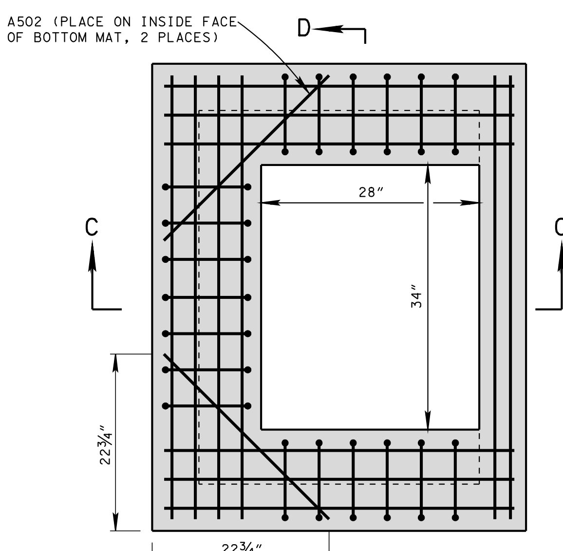
PLAN VIEW
