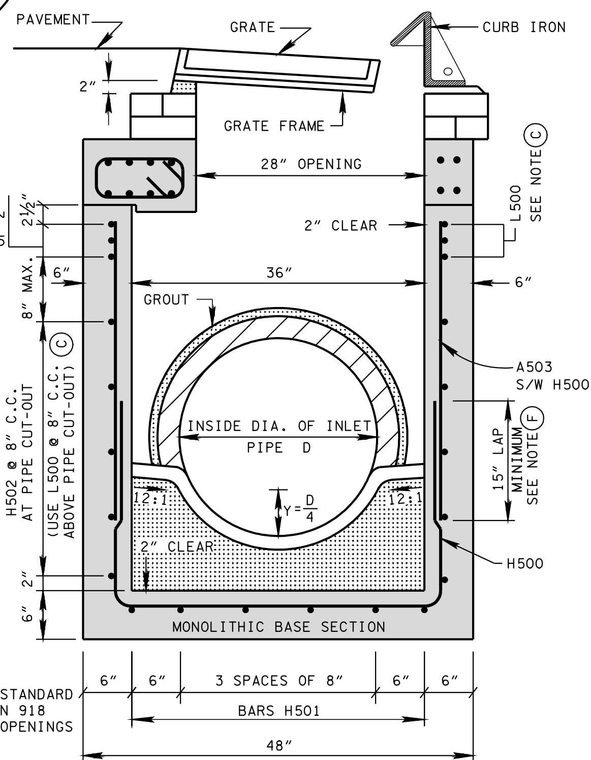
SECTION B-B
