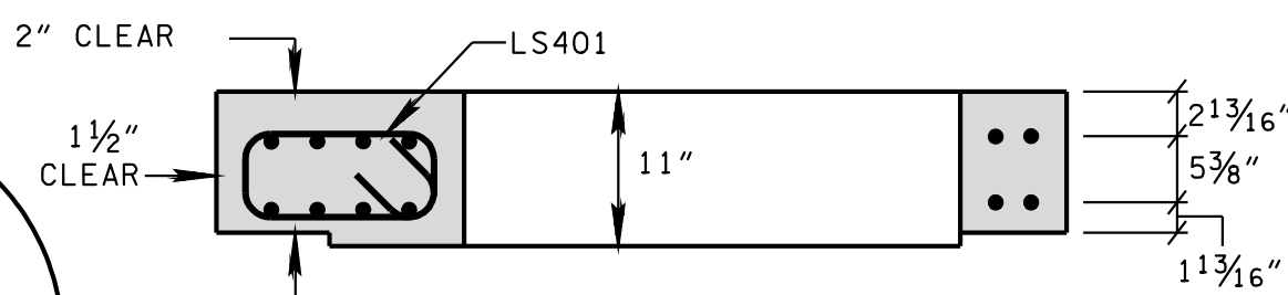
SECTION C-C
